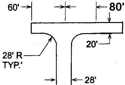
120' HAMMERHEAD
