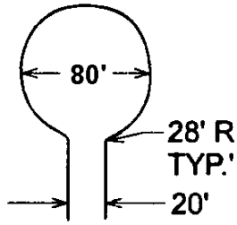
80' DIAMETER CUL-DE-SAC
