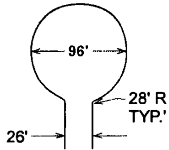
96' DIAMETER CUL-DE-SAC
